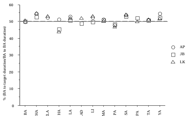
Figure 2. The amount of temporal deviation from isochrony (represented by 50%) for intervals between primary articulator velocity maxima .
