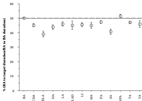
Figure 1. The amount of temporal deviation from isochrony (represented by 50%) for intervals between syllable onsets in the different syllable sequences, across six speakers. Error bars are 95% confidence intervals.
